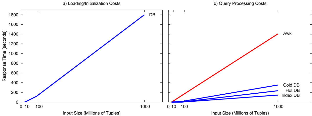
Figure 1: DB Vs. Unix tools
