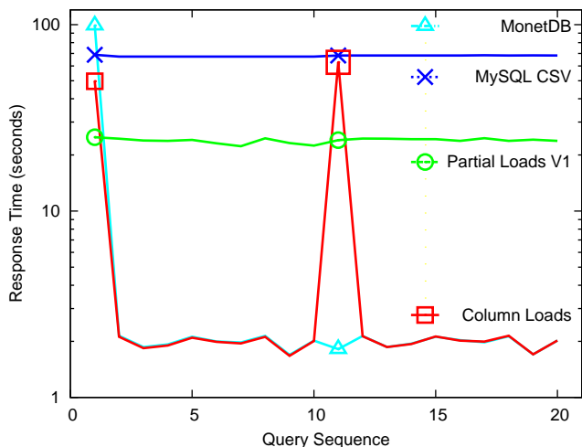
Figure 3: Alternative Loading Operators
